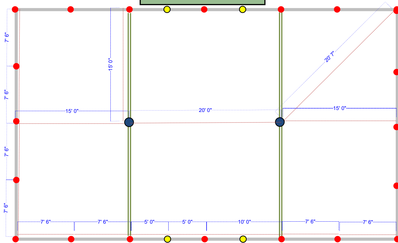
30' x 50' Pole Tent Standard & Wind - Pole placement
